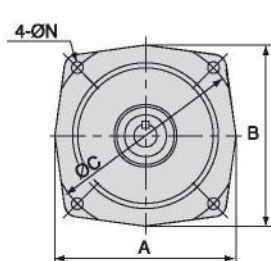
SVDL (B法蘭面) 型號Model : 11, 12, 13, 14
